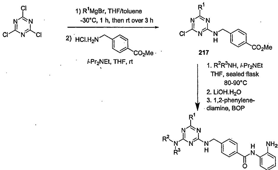
Scheme 30
